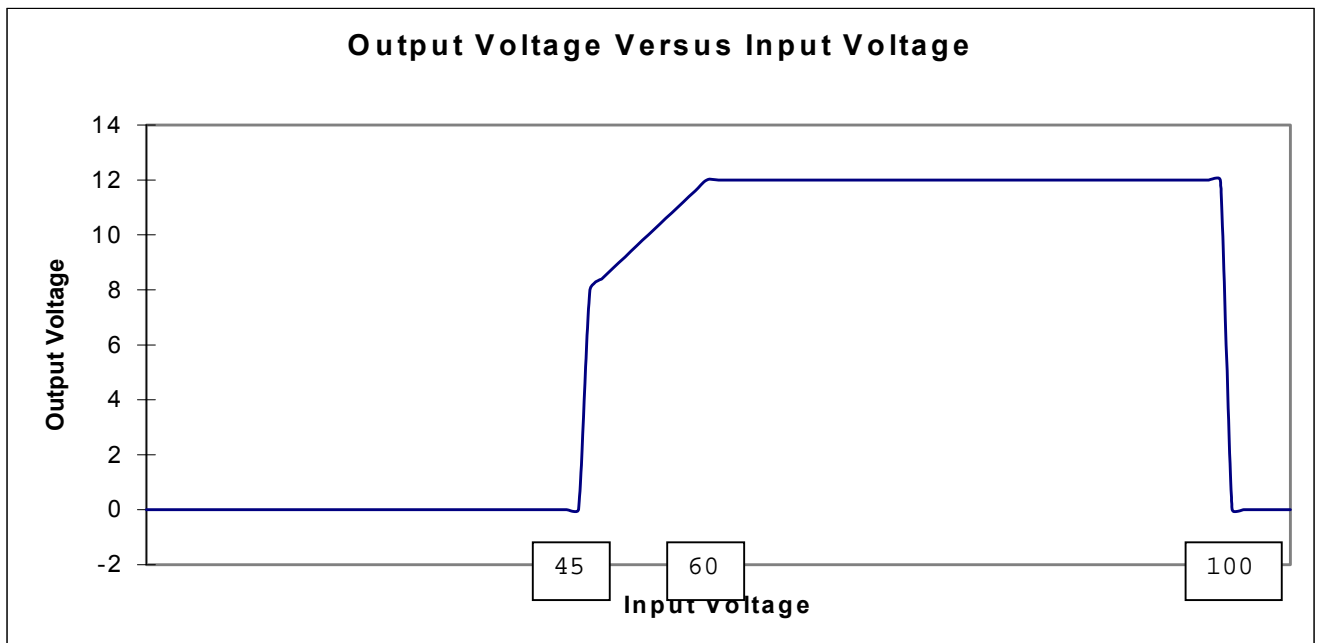
Figure 2 Output Voltage vs. Input Voltage
