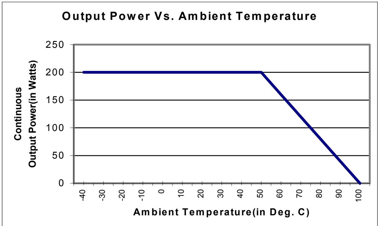
Figure 1: Temperature versus Output Power (180w unit)
