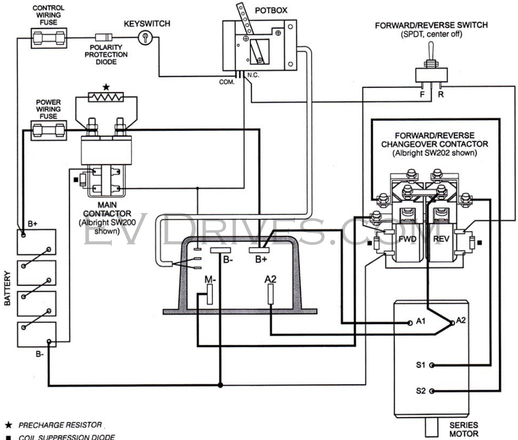
Forward Reverse Plug Brake Diagram
