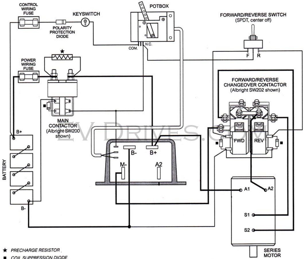
Forward Reverse No Plug Brake Diagram
